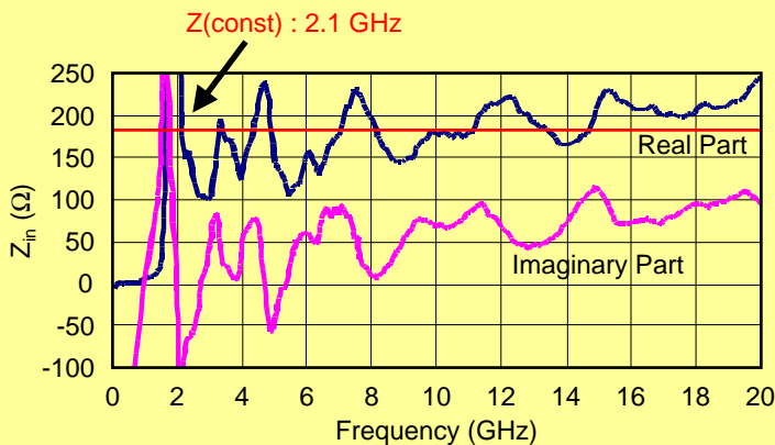
Measured input impedance (horn)
