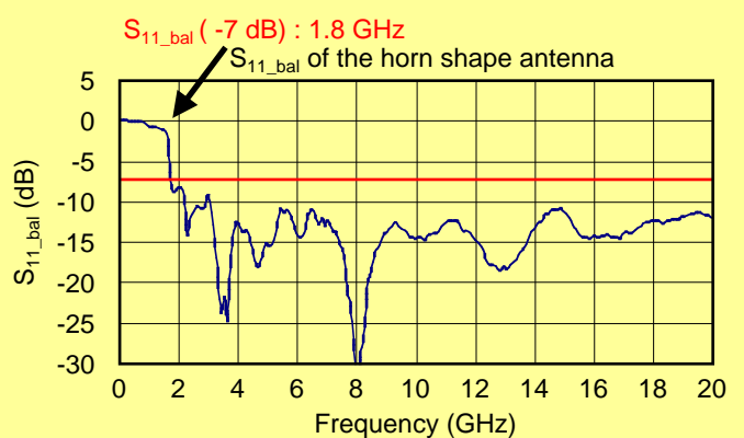
Measured Return loss for balanced input
